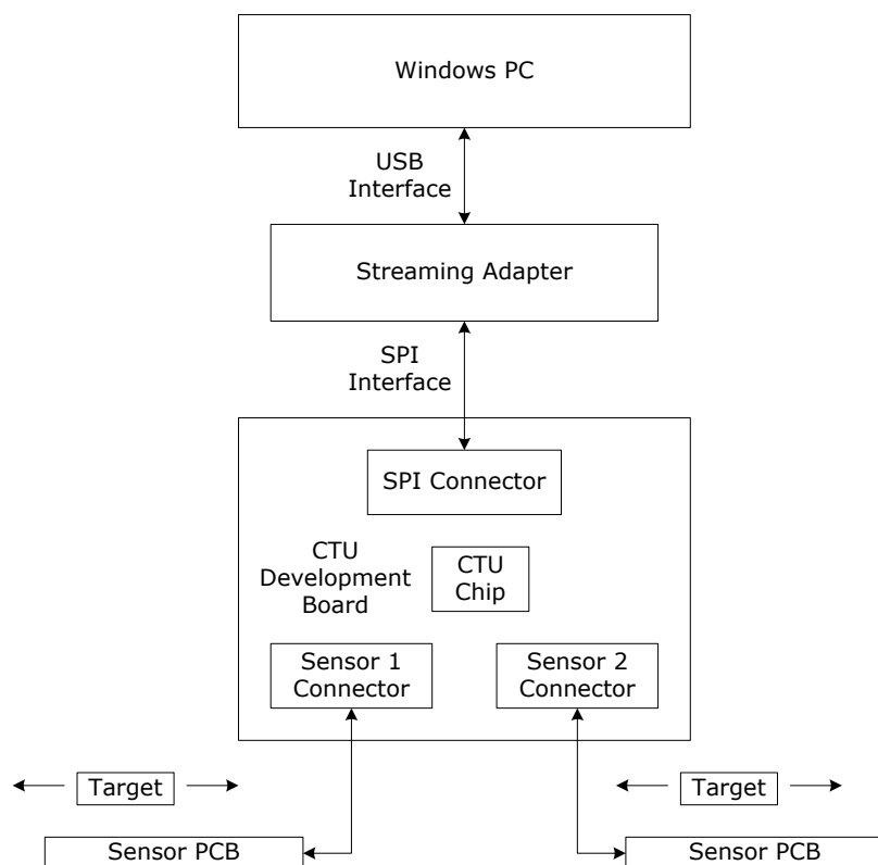
Figure 2 Hardware Connections
