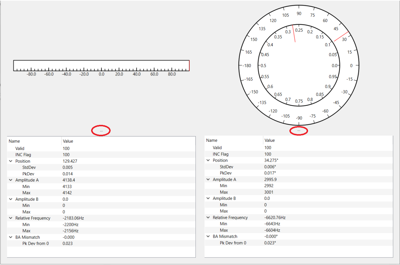
Figure 13 Digital read-outs with location of grips highlighted
