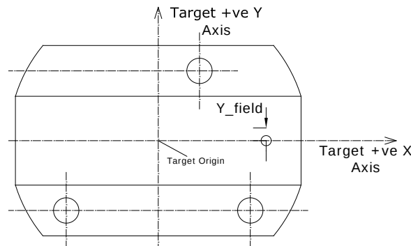
Figure 9 Y\_field measurement
