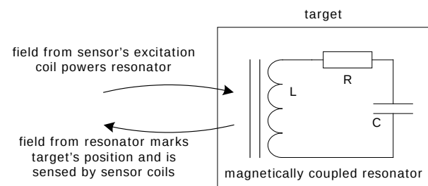
Figure 3 equivalent circuit
