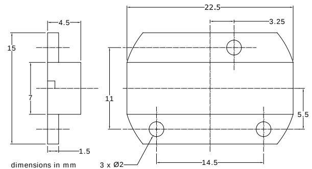
Figure 2 nominal dimensions
