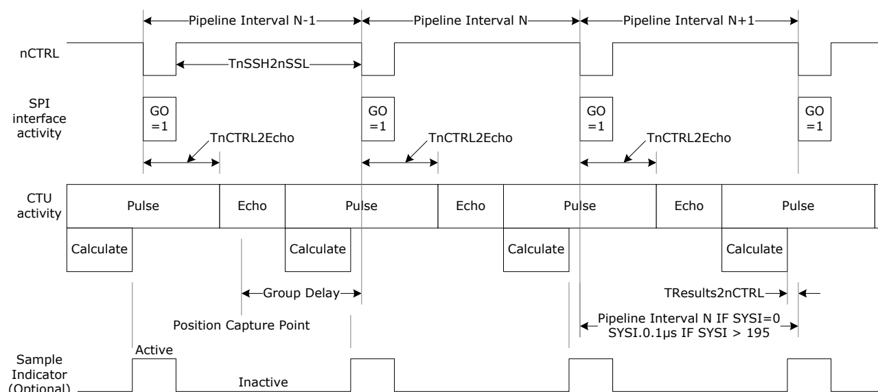
Figure 34 pipeline measurement
