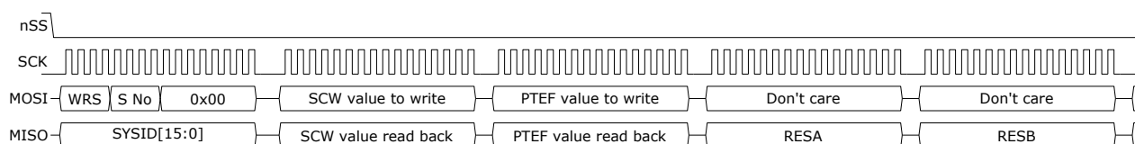
Figure 27 Write Read SPI transaction accessing SCW and measurement results, Standard SPI Format
