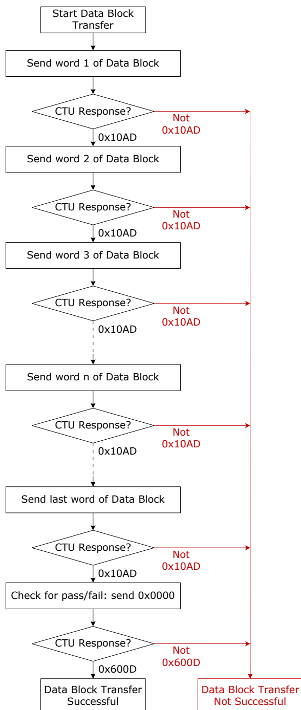
Figure 44 Data Block Transfer Process
