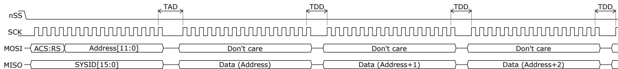
Figure 20 Multiple register access, Read
