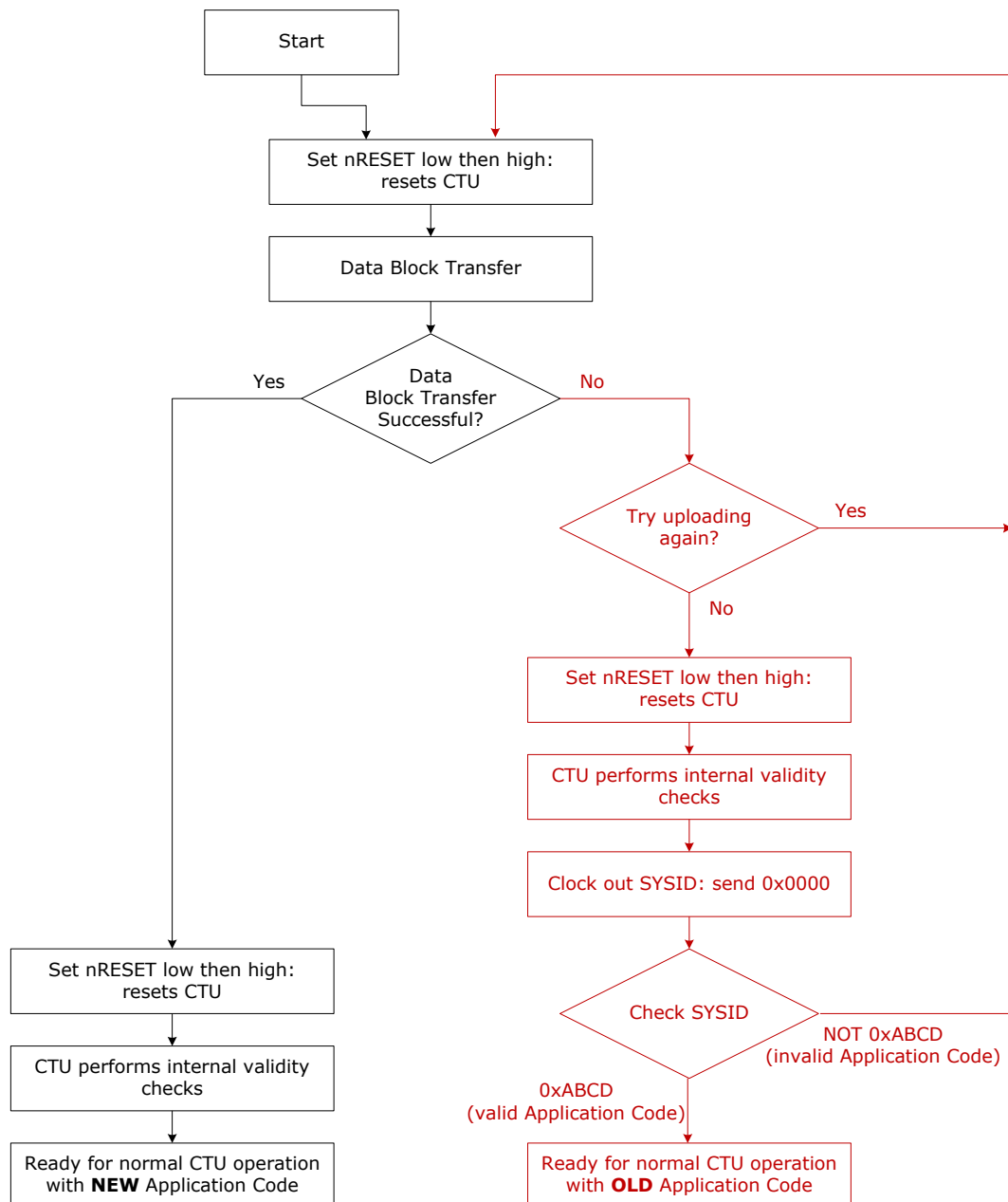
Figure 41 Bootloader Method, with nRESET
