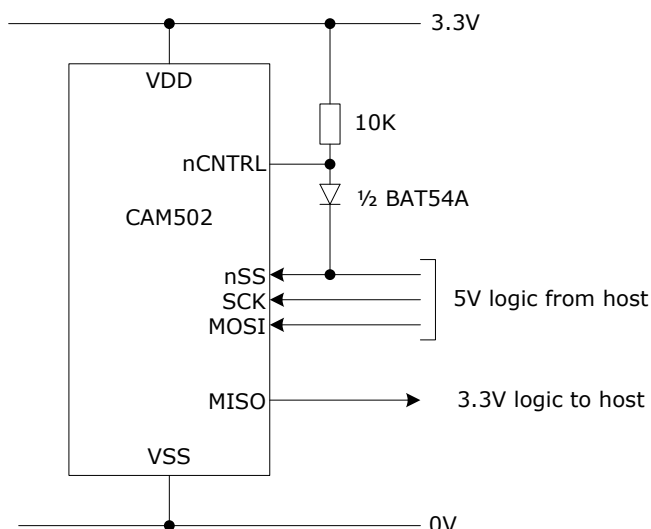
Figure 9 nCTRL level translation
