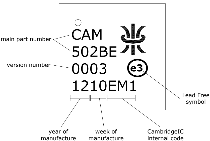
Figure 47 product markings
