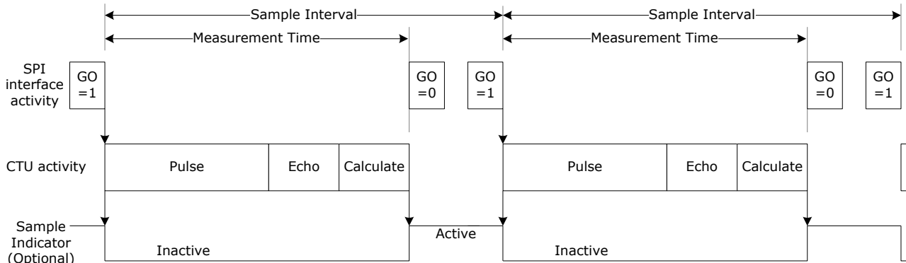
Figure 31 repeated single shot measurement, minimum delay
