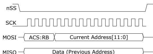
Figure 24 Burst SPI Format, Read from one register
