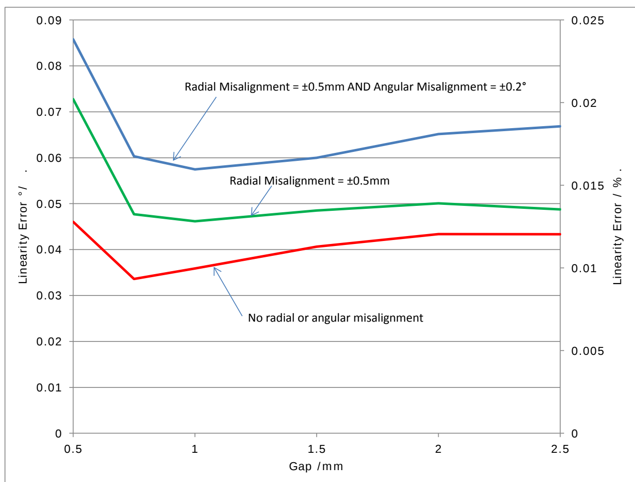
Figure 15 Linearity Error as a function of Gap and misalignment, free space
