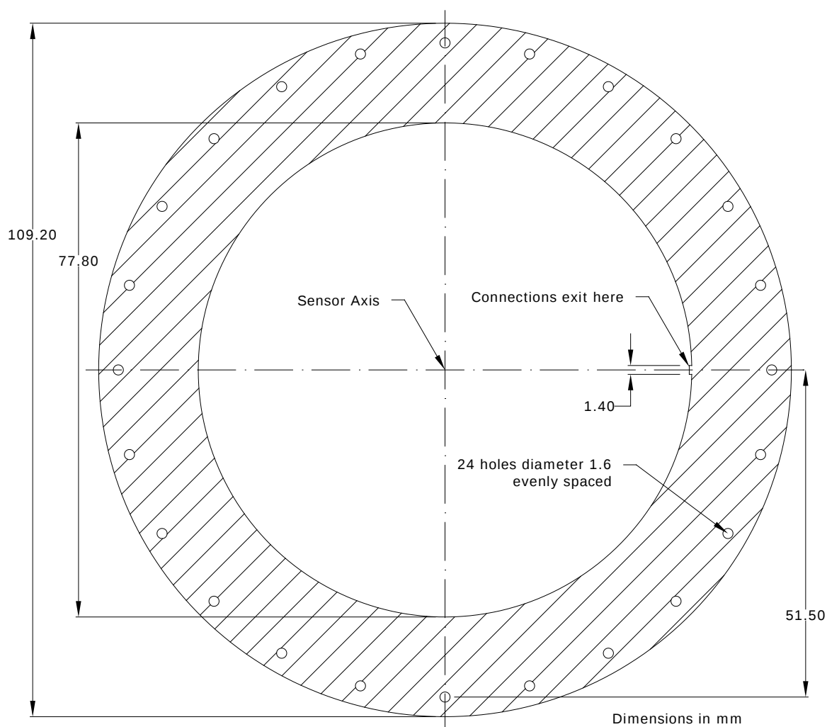
Figure 24 Copper extent
