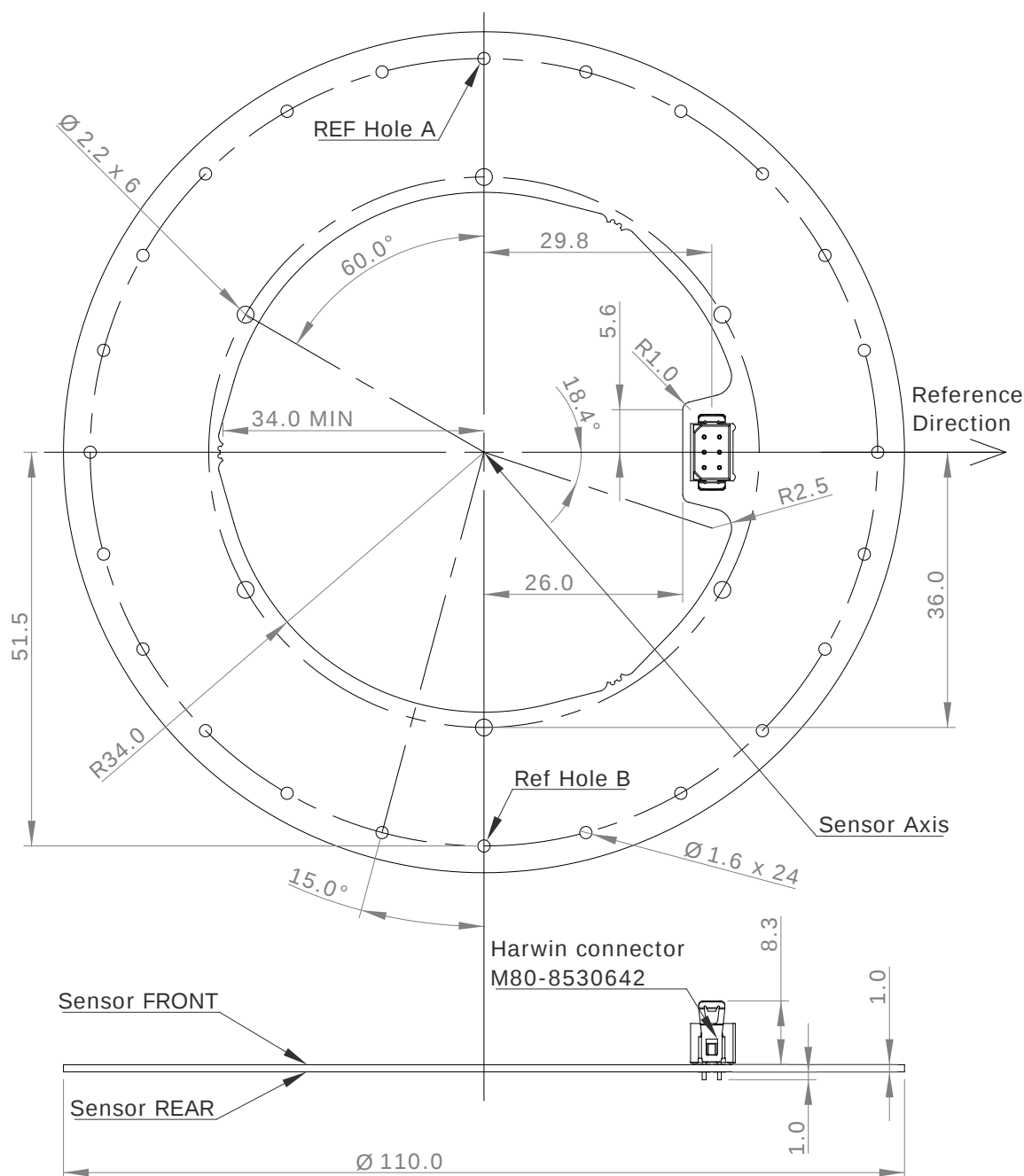
Figure 4 Assembled Sensor 013-0042
