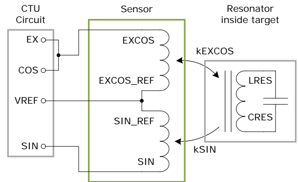
Figure 1 equivalent circuit
